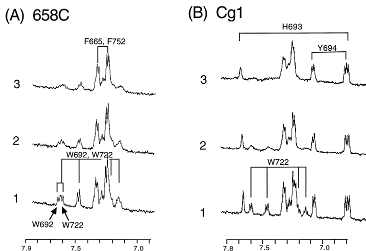
Fig. 2. Binding of 658C and Cg1 to calmodulin monitored by NMR spectroscopy. The aromatic spectral regions are shown: A: 658C: 1, 120 μM 658C; 2, 120 μM 658C+3 μM Ca 2+ -calmodulin; 3, 120 μM 658C+7 μM Ca 2+ -calmodulin. B: Cg1: 1, 160 μM Cg1; 2, 160 μM Cg1+7 μM Ca 2+ -calmodulin; 3, 160 μM Cg1+27 μM Ca 2+ -calmodulin.
